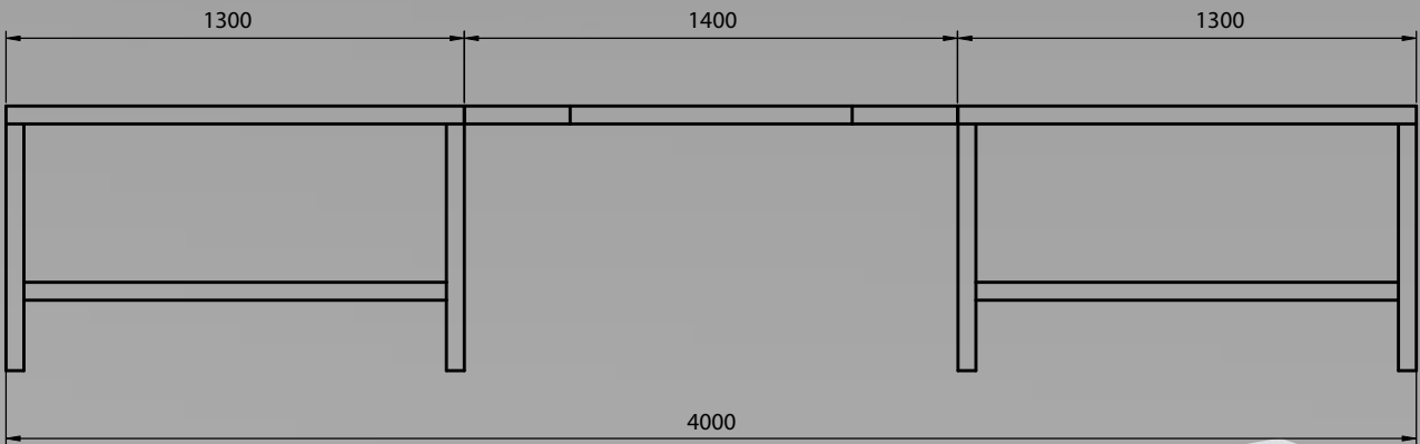
Vista frontal
