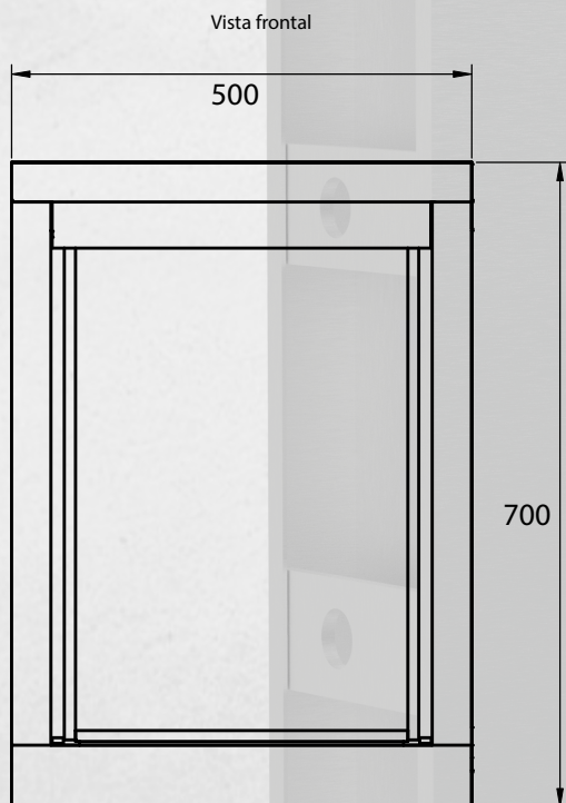
Vista frontal
